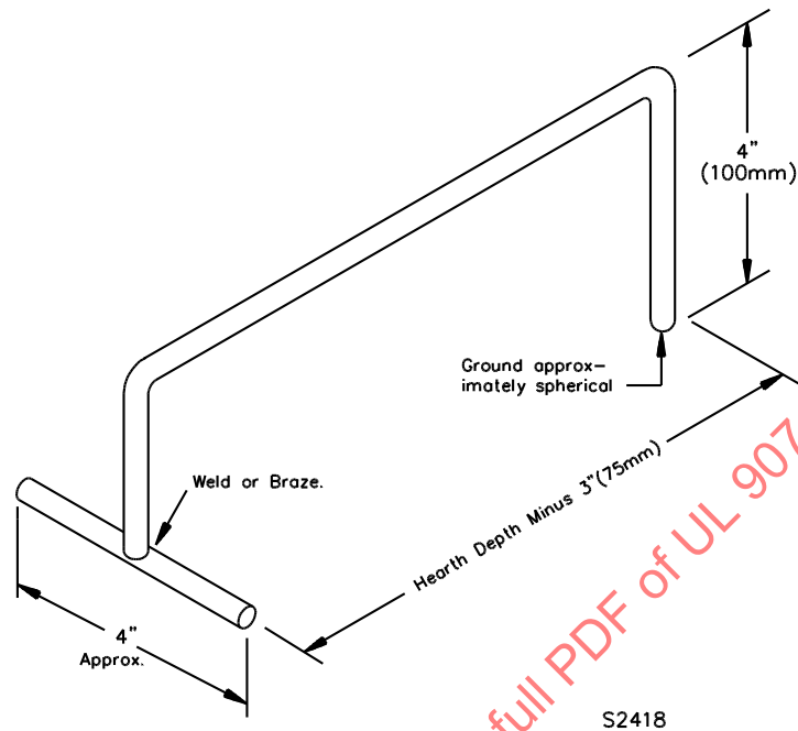
Figure 14.1 Andiron
