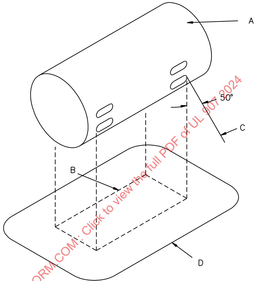
Figure 29.1 Location and Extent of Barrier
