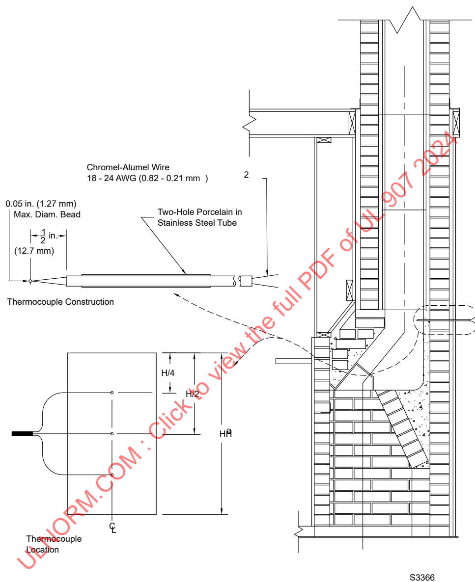
Figure 11.1 Thermocouple Location for Flue Gas Temperature Measurement
