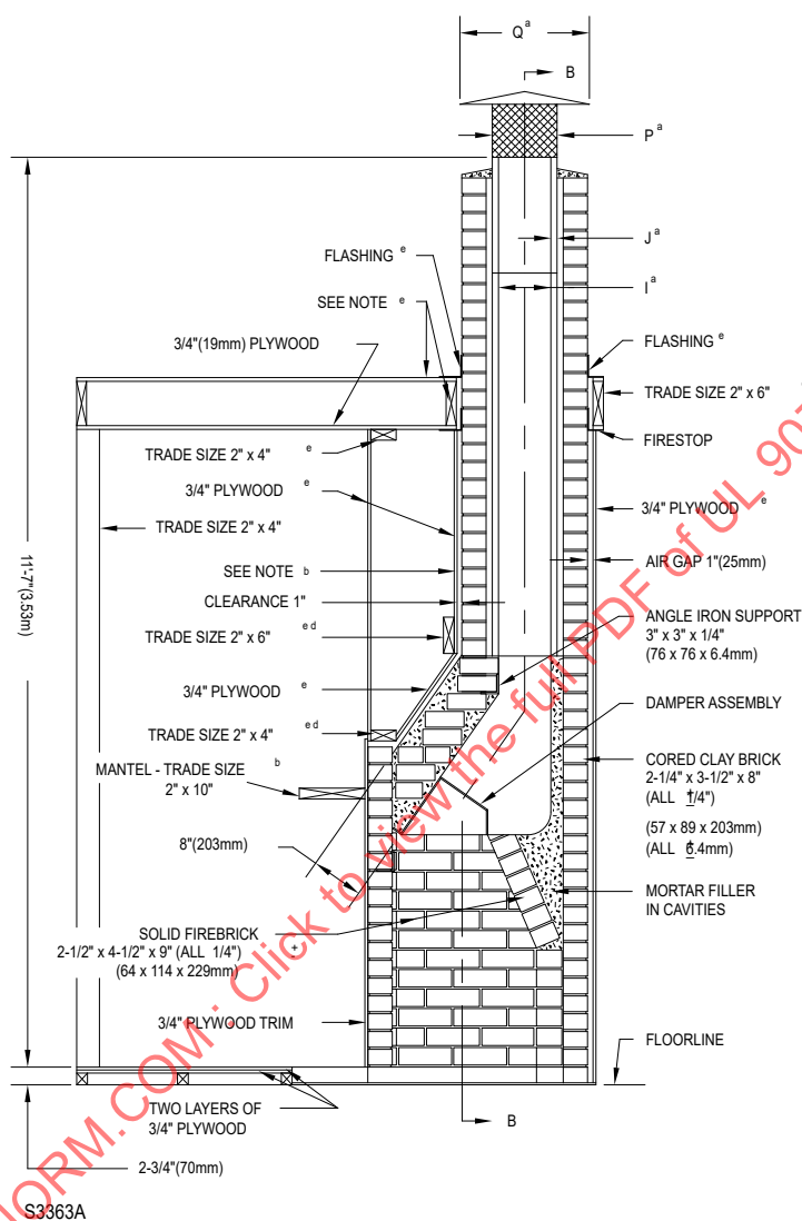
Figure 10.2 Section A – A of Figure 10.1
