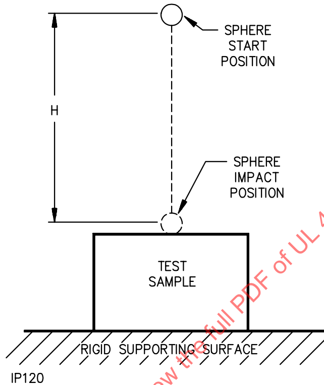
Figure 40.2 Ball Impact Tests
