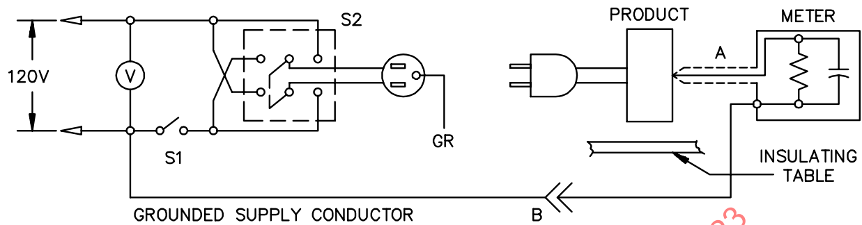
Figure 34.1 Leakage-current measurement circuit
