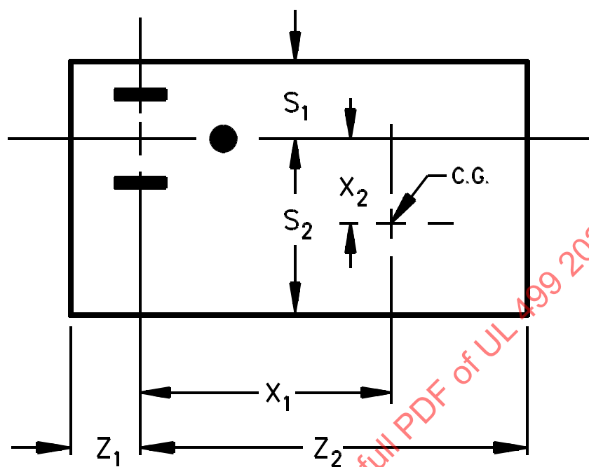
Figure 88.1 Dimensions of a direct plug-in appliance
