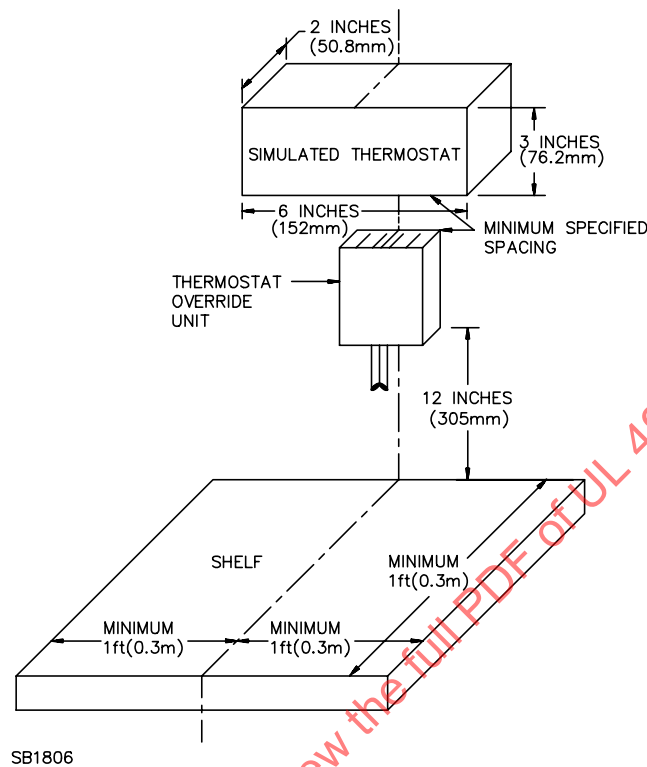
Figure 67.1 Overload test setup
