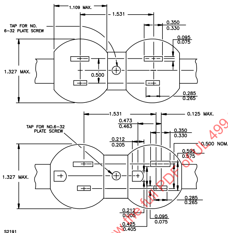
Figure 88.2 Parallel duplex receptacle
