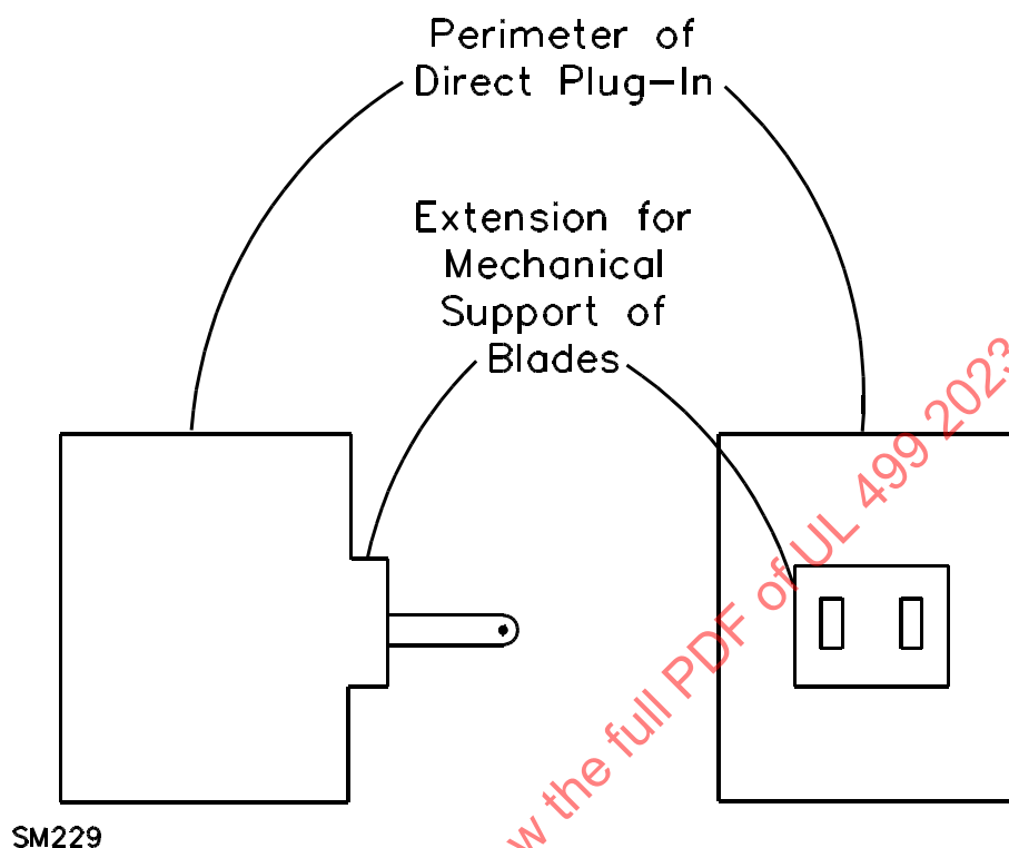
Figure 88.4 Extension for mechanical support of blades
