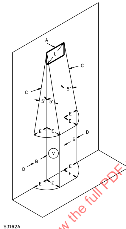
Figure 11.6 Example of Enclosure Side Opening
