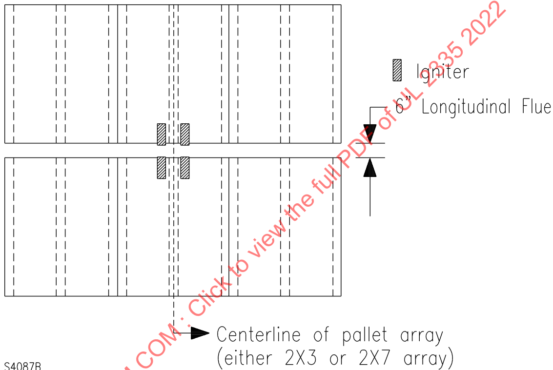
Figure 3.3 Igniter placement
