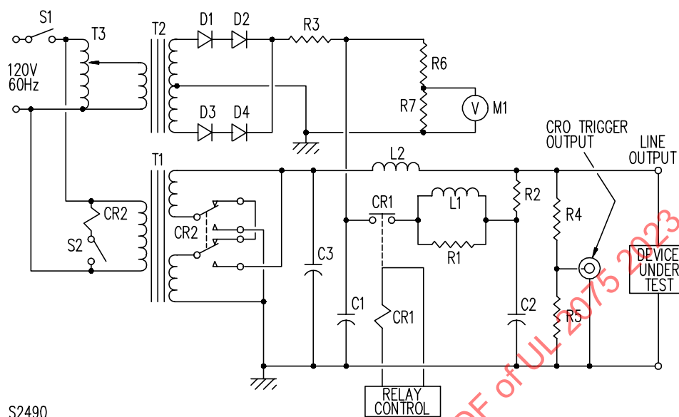
Figure 32.1 Surge generator circuit
