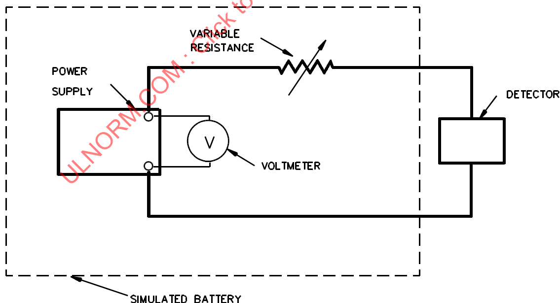
Test circuit
