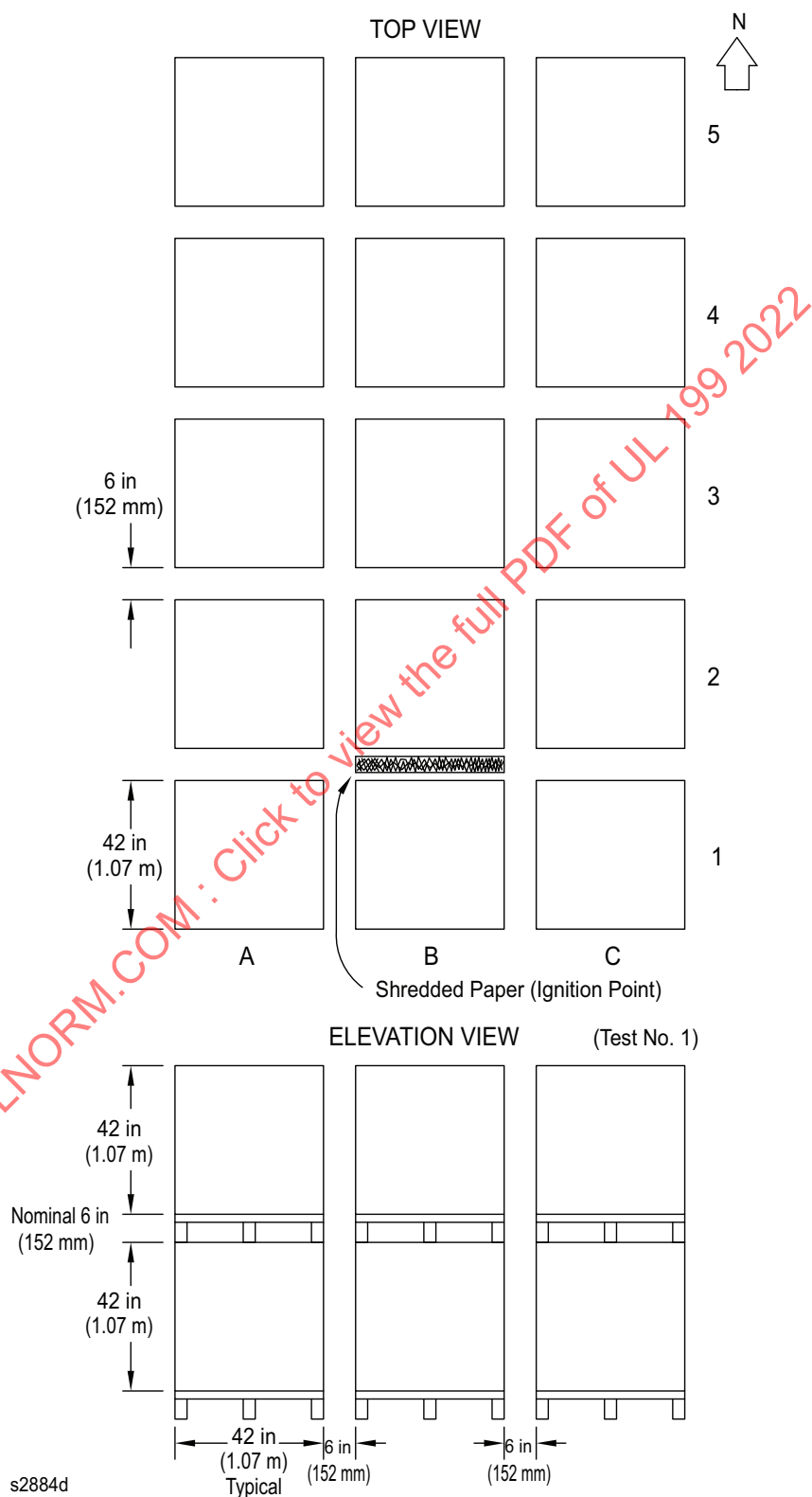
Figure 55.11 Carton Arrangement
