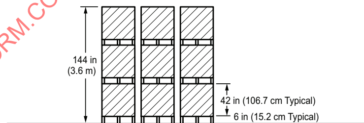
CARTON ARRANGEMENT
