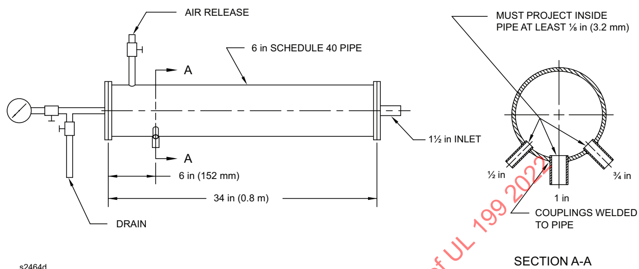
Figure 53.1 Discharge Coefficient Test Equipment
