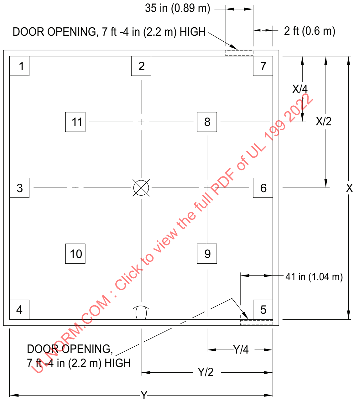
Figure 55.4 Location of Fire Test Cribbs for ECLH Sprinklers
