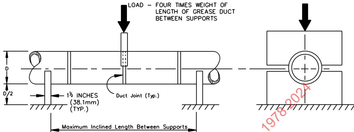
Figure 18.3 Joint load test
