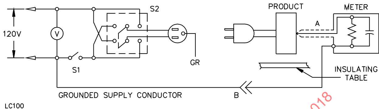
Figure 36.1 Leakage current measurement circuits
