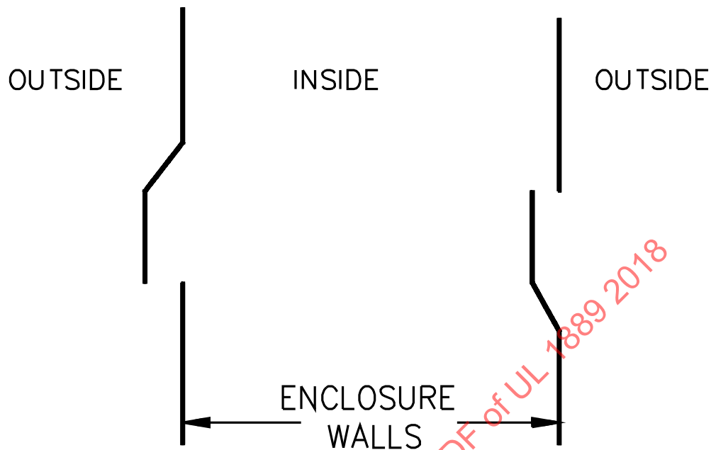
Figure 5.3 Louver constructions
