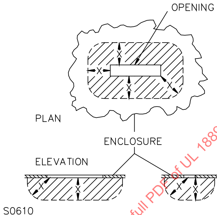
Figure 6.2 Opening in enclosure – proportions exaggerated for clarity
