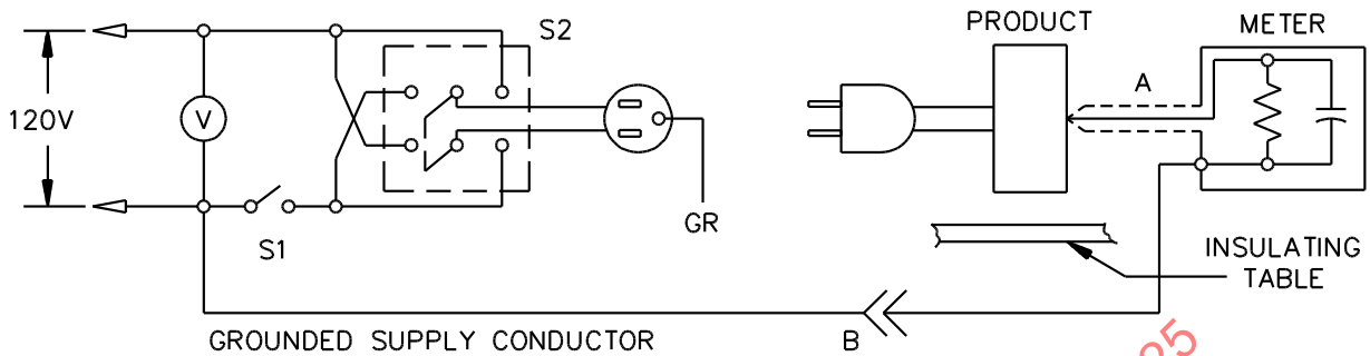
Figure 25.1 Single-phase Leakage-current Measurement Circuits
