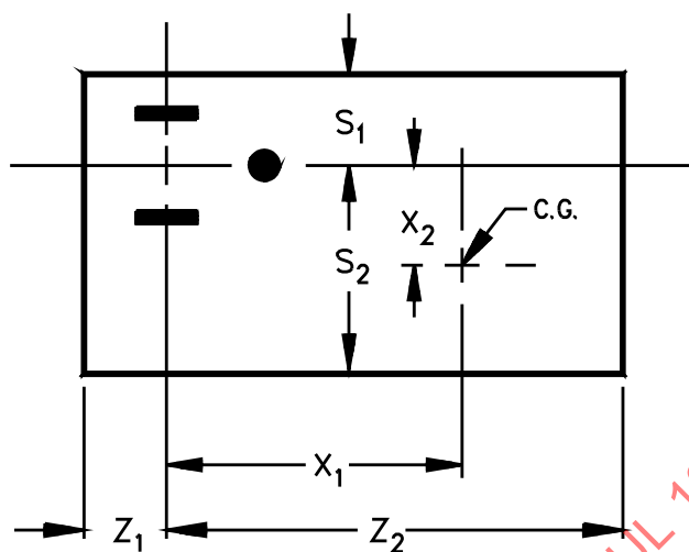
Figure 9.1 Dimensions of a Plug-in Product
