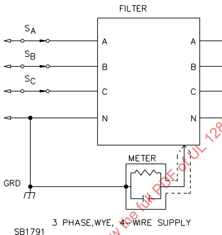
Figure 25.2 Three-phase Leakage-current Measurement Circuit
