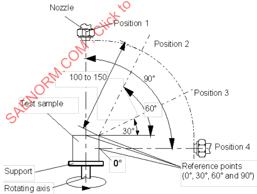
FIGURE 5.6.7.3-1: SPRAY NOZZLE AND TABLE ARRANGEMENT
