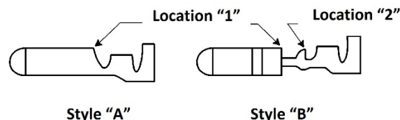
FIGURE 5.2.2.3-1: TERMINAL DESIGN STYLE
