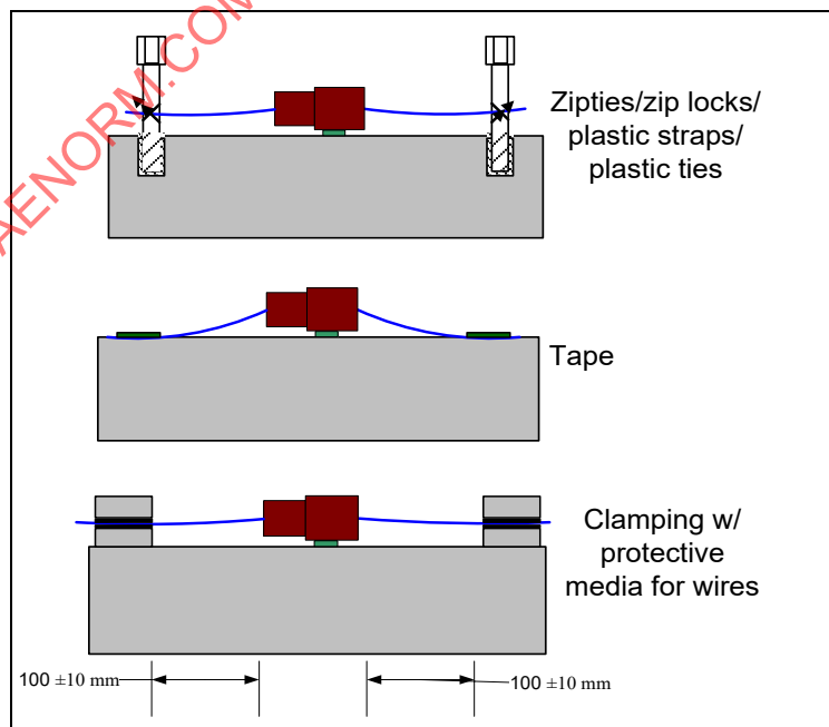
FIGURE 5.4.6.3C: TYPICAL WIRE ATTACHMENT TEST SET-UP FOR VIBRATION
