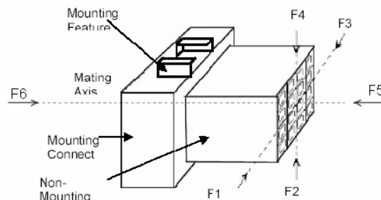
FIGURE 5.4.11.3C: TEST SET-UP (3D VIEW)
