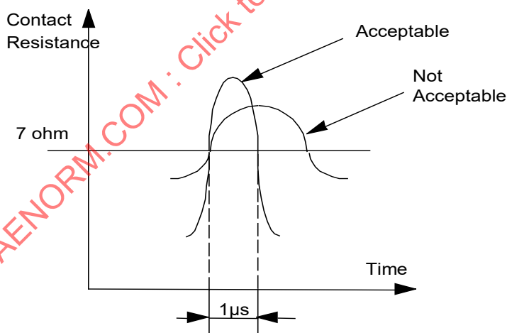
FIGURE 5.1.9.4: INTERMITTENCY MEASUREMENT
