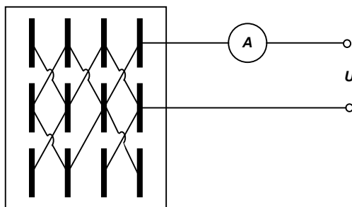
FIGURE 5.5.1.3: METHOD OF CONNECTING LEADS FOR INSULATION RESISTANCE TEST
