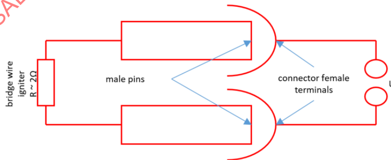
FIGURE 5.4.15.3A: CIRCUIT FOR MONITORING CONTINUITY
