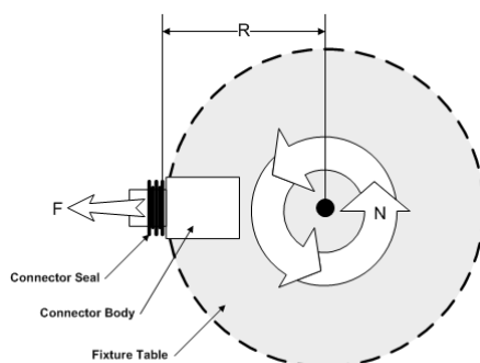
FIGURE 5.4.13.3: UNMATED CONNECTOR SEAL RETENTION TEST CONFIGURATION
