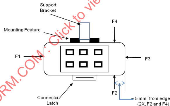
FIGURE 5.4.11.3B: TEST SET-UP (END VIEW)
