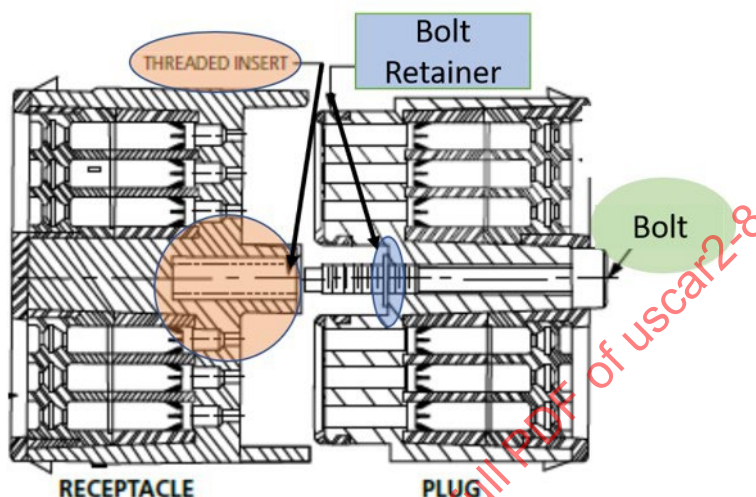
Figure 5.4.16.2: Parts of a bolted connector
