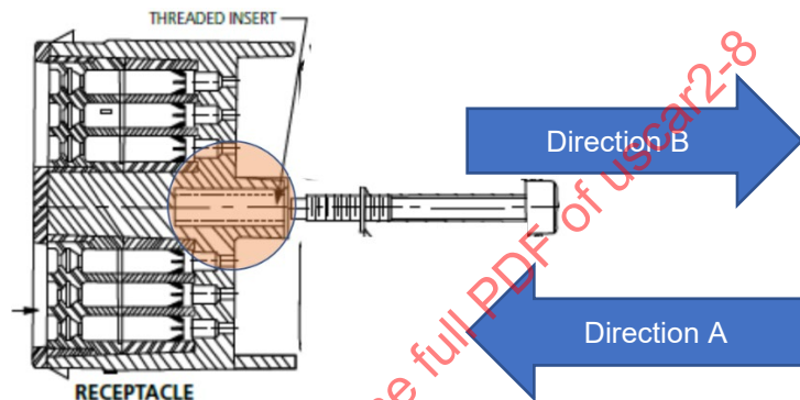
Figure 5.16.3 – Direction of force for bolt connector insert strength test
