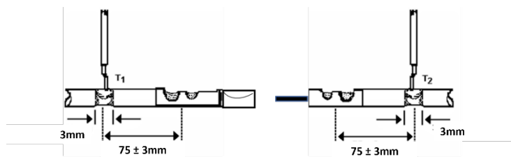
FIGURE 5.3.1.3: TYPICAL CONNECTION RESISTANCE MILLIVOLT LEAD LOCATIONS (SHOWN BEFORE MATING TERMINALS OR INSERTING TERMINAL INTO CONNECTOR)
