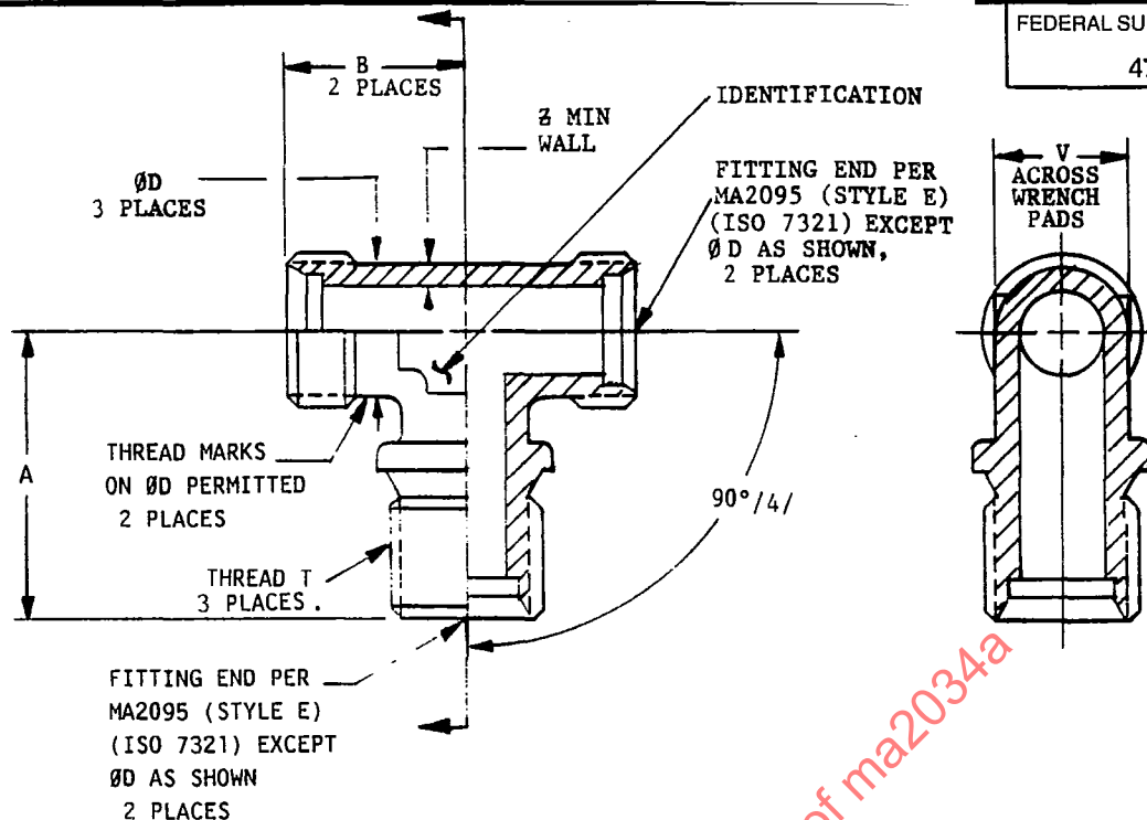
FIGURE 1 - FRONT AND SIDE VIEWS
