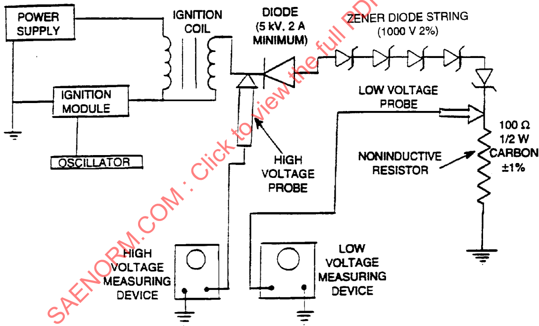
FIGURE 4—IGNITION COIL ENERGY MEASUREMENT (ZENER TECHNIQUE)
