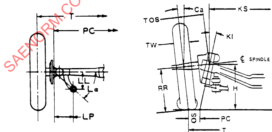
FIGURE 2—DIAGRAM ILLUSTRATING FACTORS OF FRONT AXLE CONFIGURATION
