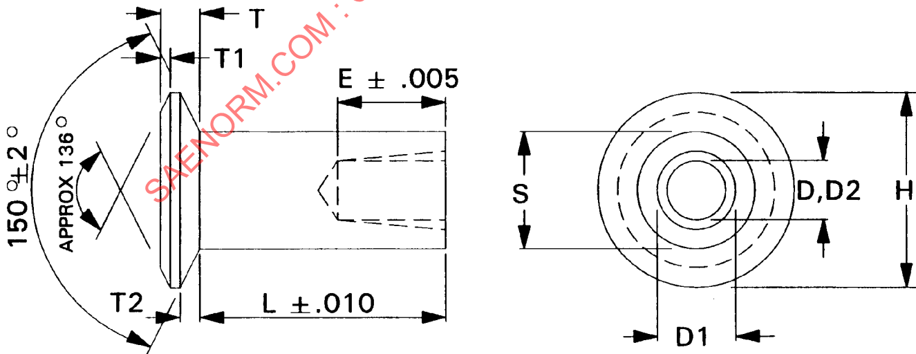
FIGURE 1—SEMITUBULAR RIVET FOR BRAKE LININGS/BLOCKS
