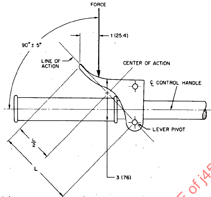
NOTE: DIMENSIONS ARE IN (mm) FIG. 1
