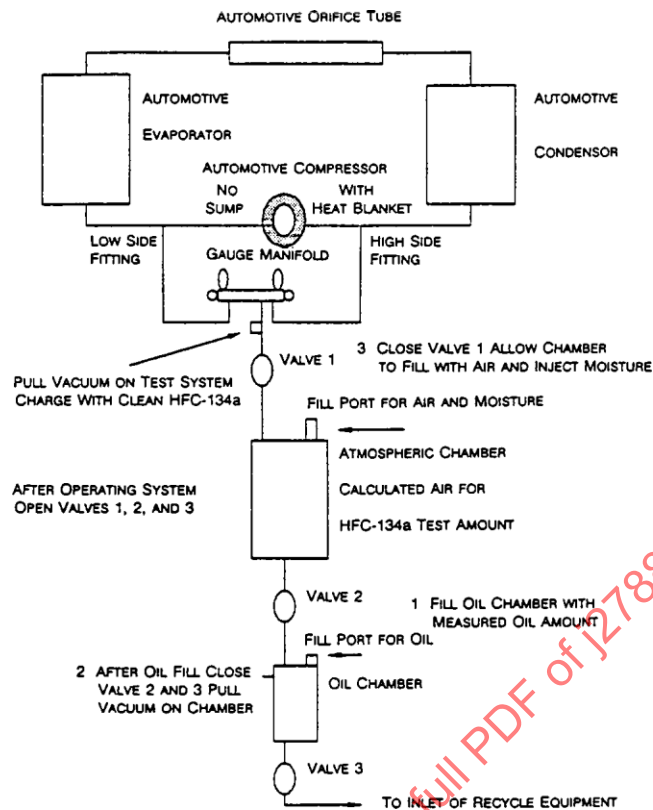
FIGURE 1 -TEST FIXTURE
