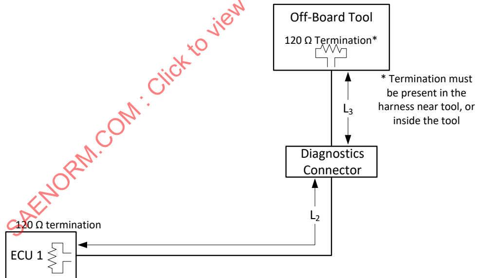
Figure 2 - Single on-board ECU configuration B
