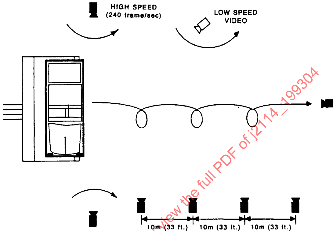
FIGURE 2—PHOTOGRAPHIC COVERAGE (NOTE—2 ONBOARD CAMERAS NOT SHOWN)
