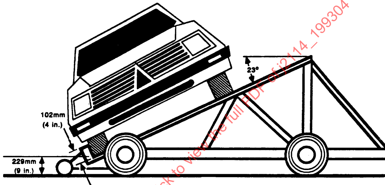
FIGURE 1—DOLLY ROLLOVER FIXTURE
