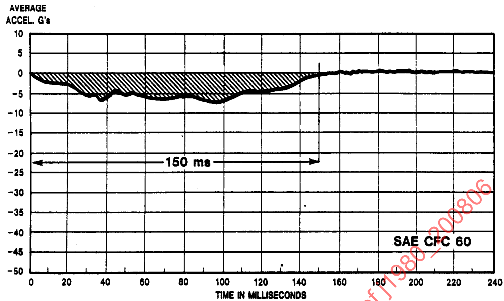
FIGURE 1—GENERIC HYGE SLED PULSE FOR A MILD CRASH SEVERITY
