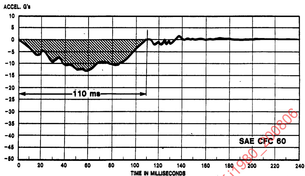
FIGURE 3—GENERIC HYGE SLED PULSE FOR A MODERATE CRASH SEVERITY
