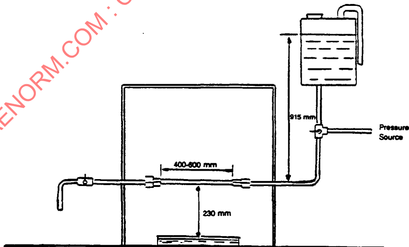
FIGURE 2—TEST SET-UP
