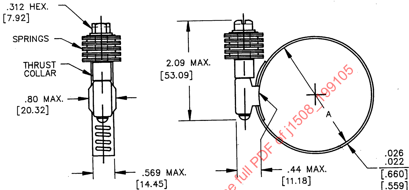
FIGURE 19—TYPE "SLF"—INCH [METRIC]
