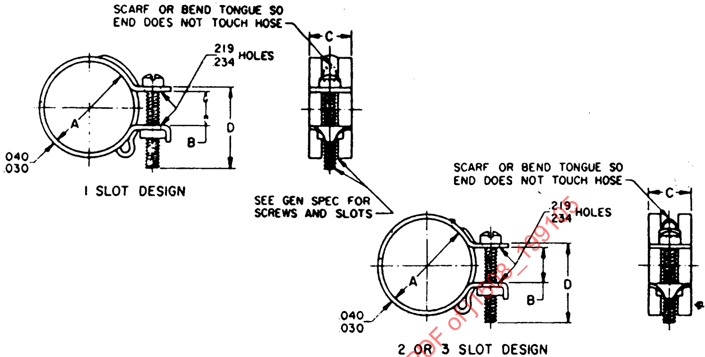
FIGURE 2—TYPE "B" HOSE CLAMPS
