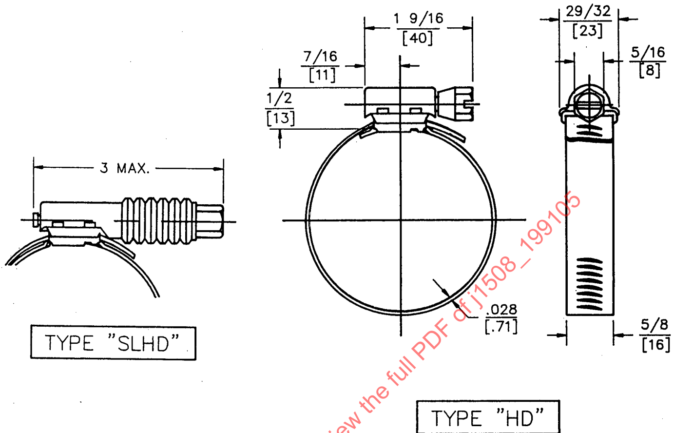
FIGURE 11—TYPE "HD" AND "SLHD"
