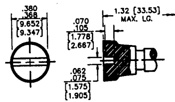
OPTIONAL DESIGNS STYLE 1
