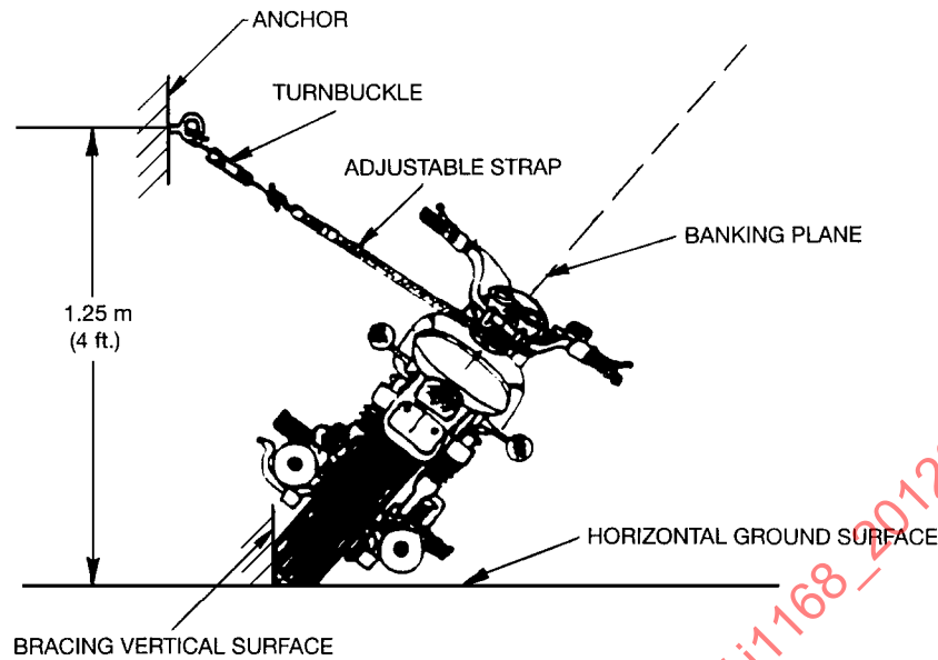
FIGURE 1—PROCEDURE SET-UP
