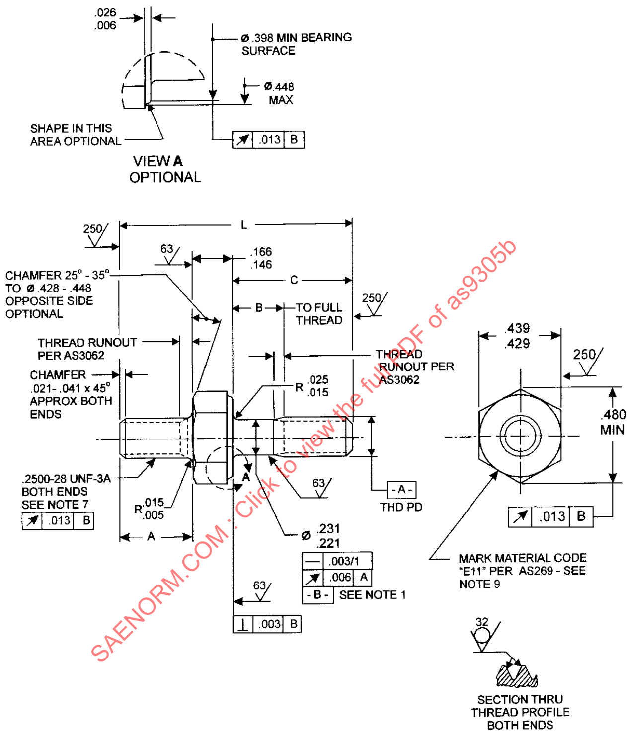
FIGURE 1 – STUD
