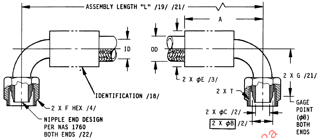
FIGURE 1 - HOSE ASSEMBLY
