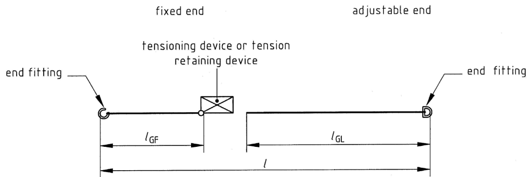
FIGURE 2 - TWO-PIECE RESTRAINT STRAP ASSEMBLY
