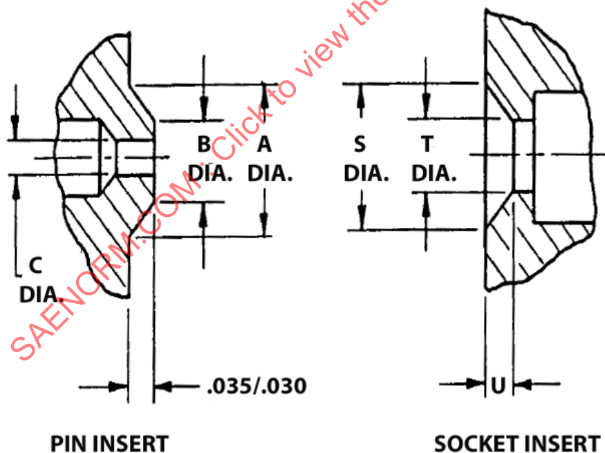
Figure 6 - Connector, rear release, series III, insert entry dimensions
