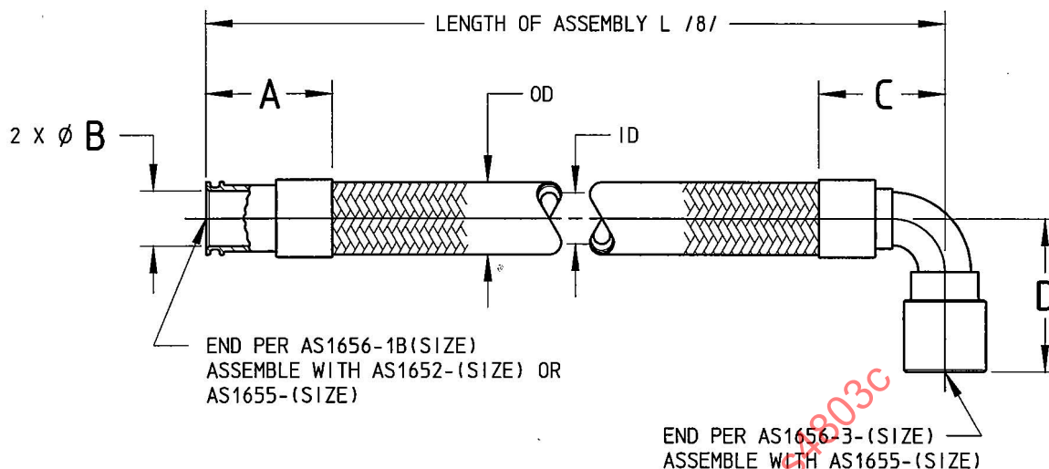
FIGURE 1 - HOSE ASSEMBLY
