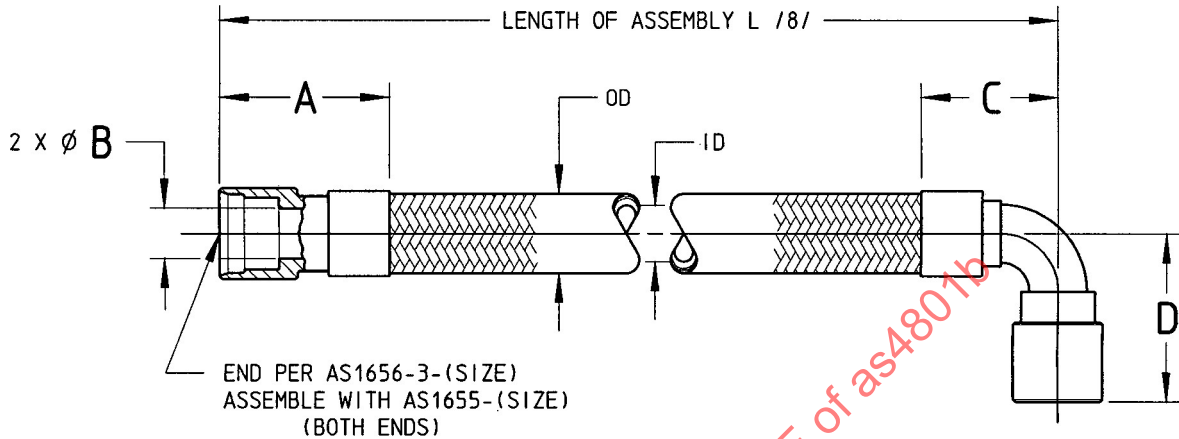
FIGURE 1 - HOSE ASSEMBLY
