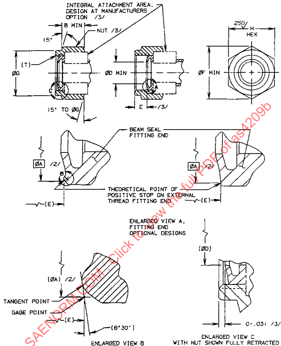
(R) FIGURE 1 - FITTING END DESIGN WITH LIMITS OF NUT TRAVEL
