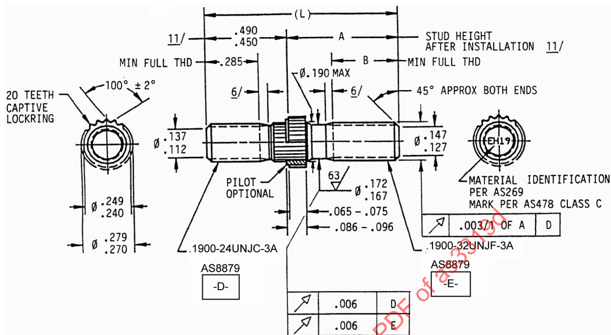
FIGURE 1 - STUD
