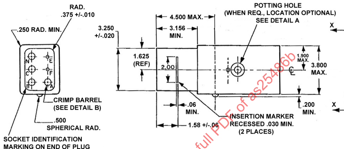
FIGURE 1 - AS25486 ATTACHABLE PLUG CONFIGURATIONS
