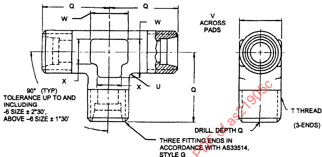
FIGURE 1 - TEE, FLARELESS TUBE
