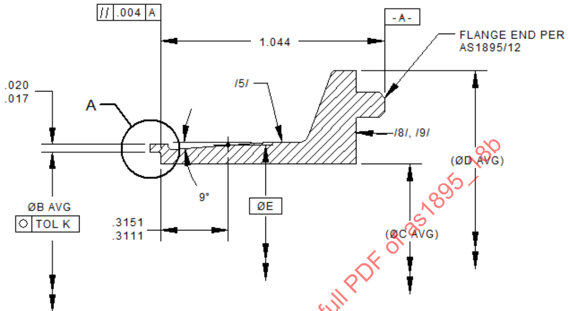
FIGURE 1 - TYPICAL SECTION
