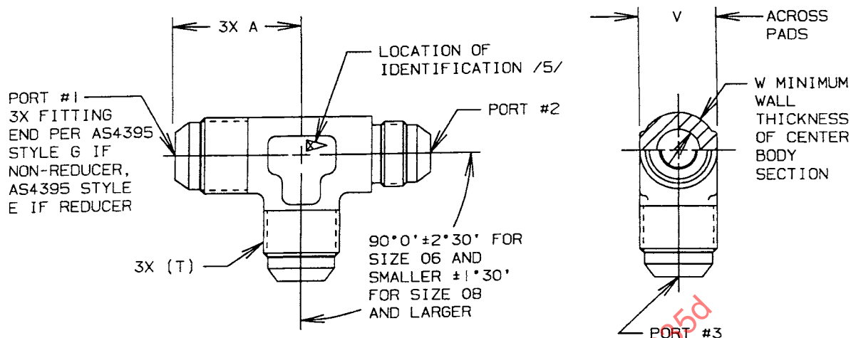
FIGURE 1 - TEE, FLARED
