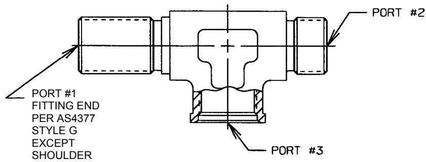
FIGURE 3 - FITTING, TEE, BULKHEAD END NOT FOR USE IN PORT INSTALLATION, PORT #3 SHOWN AS NON-REDUCER, SAME AS FIGURE 1 EXCEPT AS SHOWN
