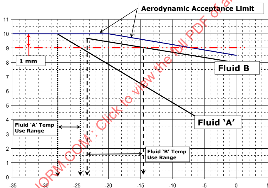
Figure D1 - Anti-icing fluid temperature use evaluation
