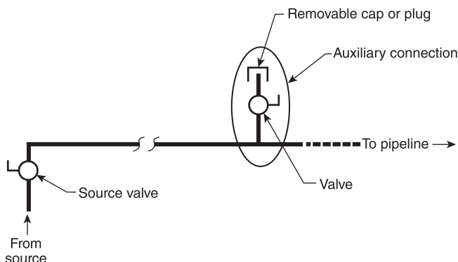
FIGURE A.5.1.3.5.14 Typical Configuration of an Auxiliary Connection.
