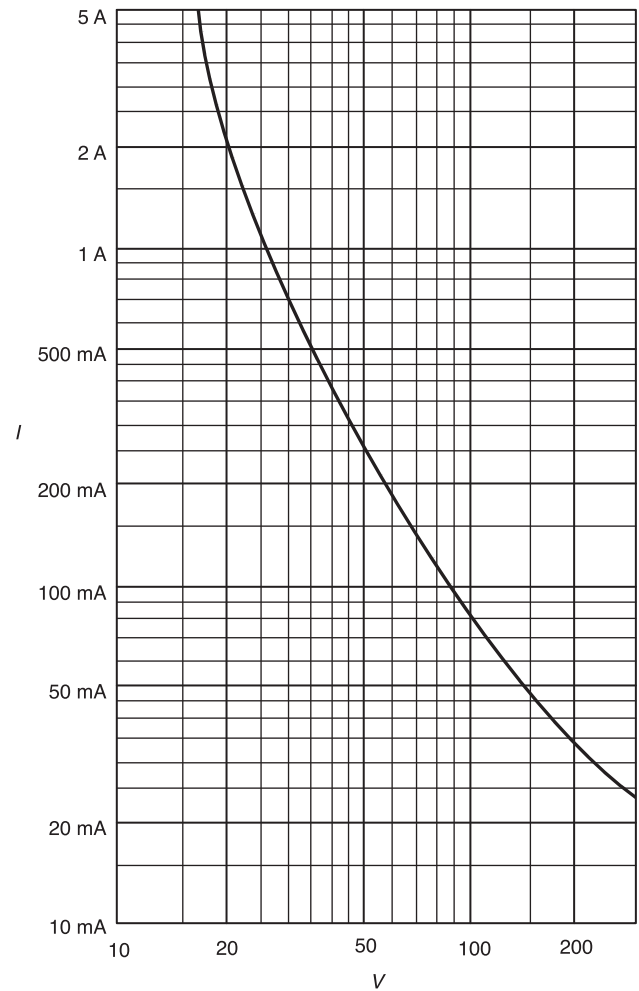
FIGURE 10.5.4.1(a) Resistance Circuits ( L < 1 \text{ mH} ): Minimum Igniting Currents, Applicable to All Circuits Containing Cadmium, Zinc, or Magnesium.
