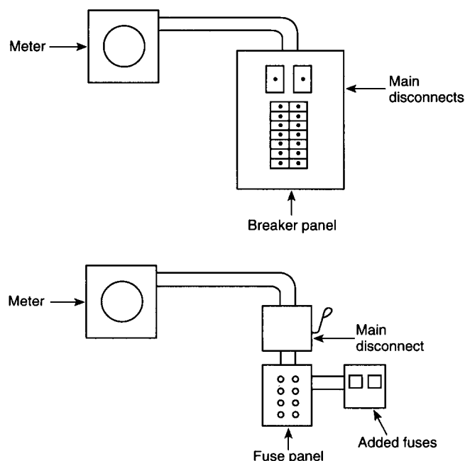
Figure 14-3.1.2 Service equipment.
