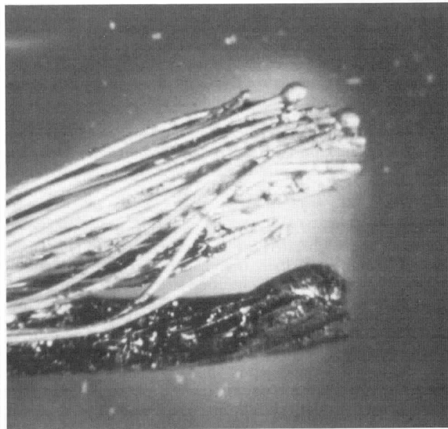
Figure 14-5.3 Stranded copper lamp cord that was severed by a short circuit.
