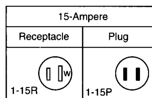
Figure 14-3.10(a) Nongrounding type.
