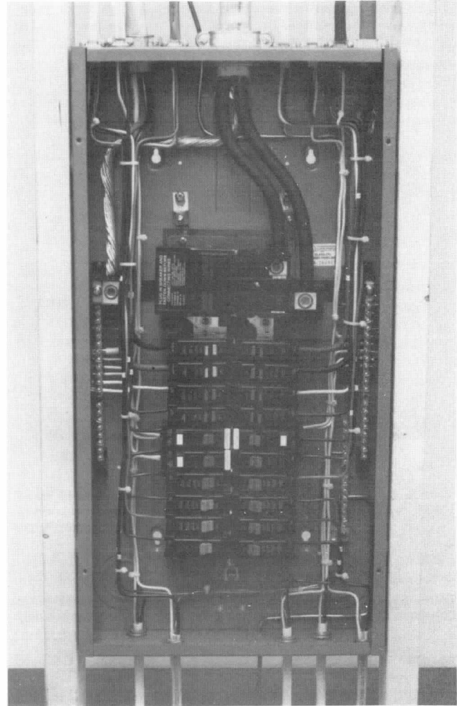
Figure 14-3.3.2(c) Photograph of a circuit-breaker panel.
