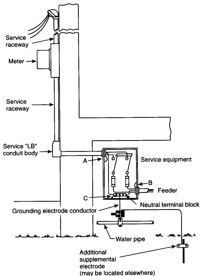
Figure 14-3.2.3 Grounding at a typical small service. A, B, and C are bonding connections that provide a path to ground.
