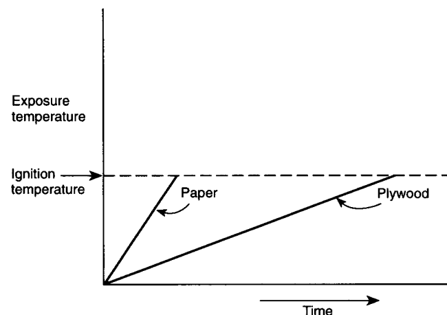
Figure 3-3.1(b) Relationship of material thickness to ignition time when exposed to ignition temperature.
