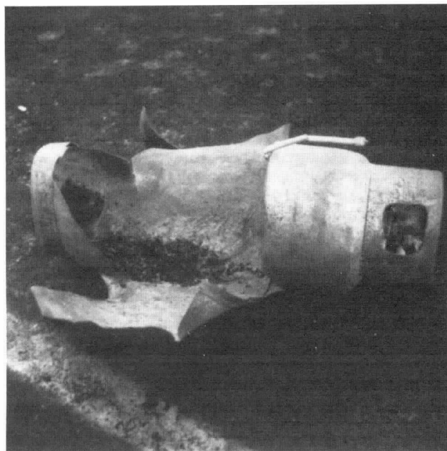
Figure 13-2.1.1(a) An LP-Gas cylinder that suffered a BLEVE as a result of exposure to an external fire.
