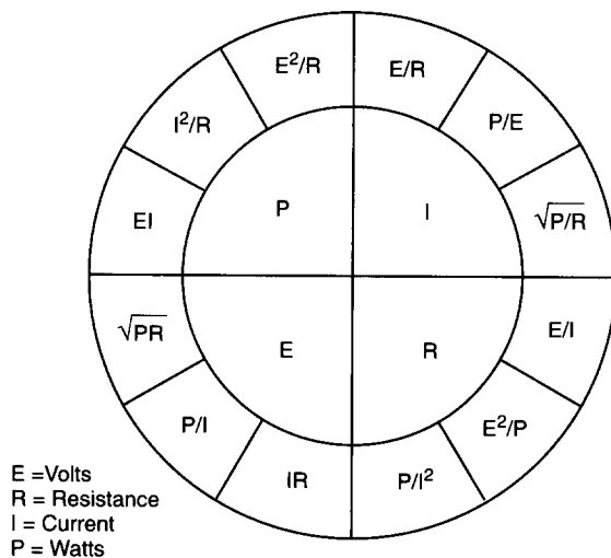
Figure 14-2.15 Ohms Law wheel resistive circuits.
