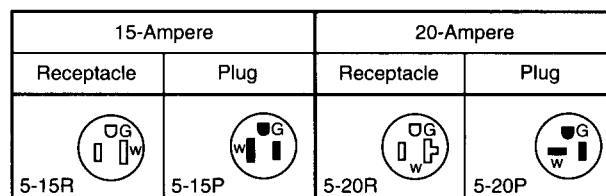
Figure 14-3.10(b) Grounding type.
