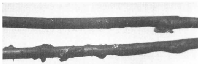
Figure 14-6.2(a) Copper conductors, fire-heated to the melting temperature, showing regions of flow of copper, blistering, and no surface distortion.
