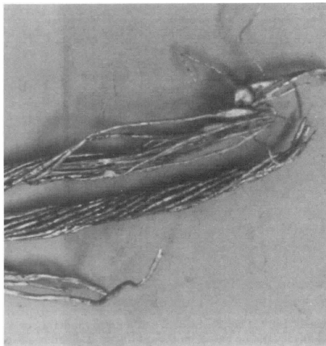
Figure 14-6.2(d) Aluminum cables that were melted by fire showing thinned areas, bulbous areas, and pointed ends.
