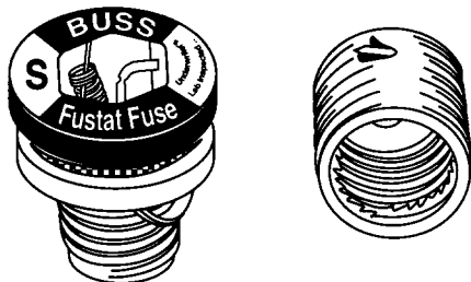
Figure 14-3.5(c) A Type S nonrenewable fuse. The time lag type of fuse is acceptable but not required. These fuses have been designed so that tampering or bridging can be done only with difficulty. NFPA 70, National Electrical Code , specifies that fuse holders for plug fuses of 30 amperes or less shall not be used unless they are designed to use this Type S fuse or are made to accept a Type S fuse through use of an adapter. (Bussmann Division, Cooper Industries)
