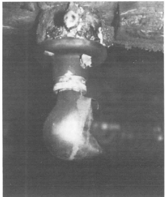
Figure 4-20.1 A typical “pulled” bulb showing that the heating was from the right side.
