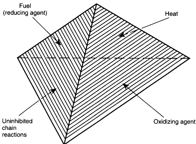
Figure 3-1.1 The tetrahedron of fire.
