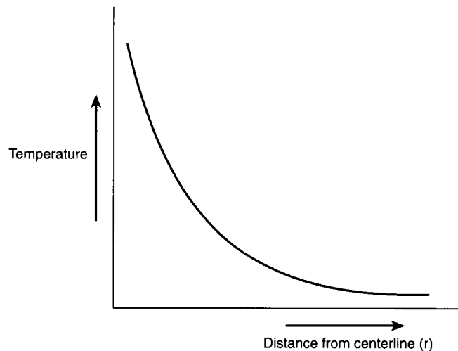
Figure 3-5.3.1(b) Ceiling layer temperature away from the plume.
