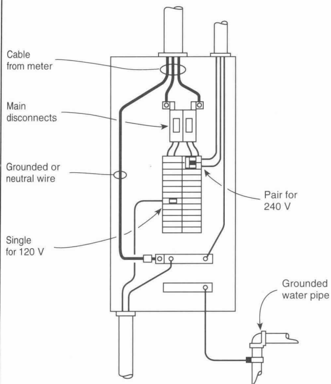
Figure 14-3.3.2(b) Common arrangement for a circuit-breaker panel.
