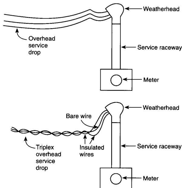
Figure 14-3.1.1(a) Overhead service.
