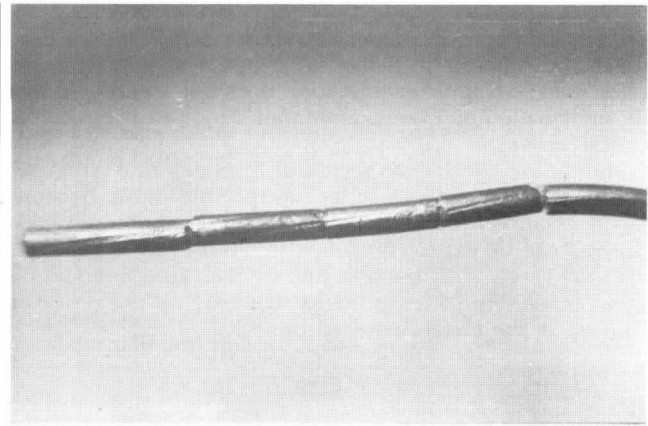
Figure 14-5.6 Aluminum conductors severed by overcurrent showing offsets.
