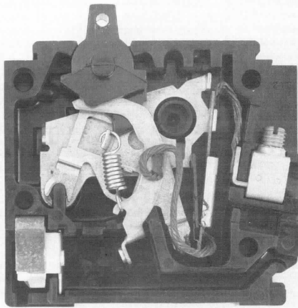
Figure 14-3.5.3.1(d) A 15-ampere residential-type circuit breaker in the open (tripped) position. (Challenger Electrical Equipment Corp., subsidiary of Westinghouse Electric Corp.)
