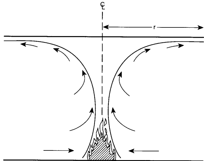
Figure 3-5.3.1(a) Fire confined by a ceiling in a large room.
