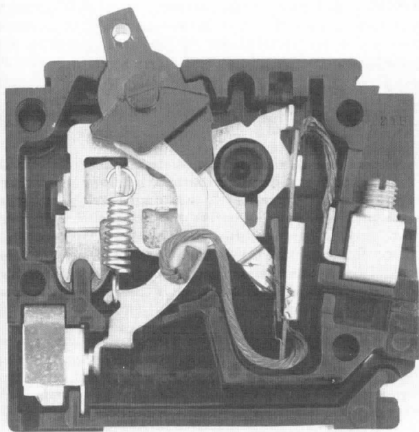
Figure 14-3.5.3.1(b) A 15-ampere residential-type circuit breaker in the closed (on) position. (Challenger Electrical Equipment Corp., subsidiary of Westinghouse Electric Corp.)
