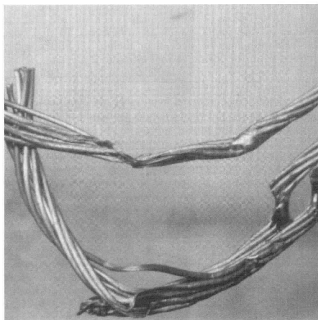
Figure 14-6.2(e) Aluminum cables that were melted by fire while partly protected in conduit.
