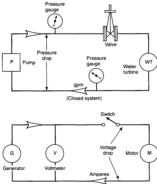
Figure 14-2.8 Water pressure is measured by a pressure gauge. Voltage is measured by a voltmeter. A valve is used to turn water on and off. A switch is used to turn the electricity to a motor on and off. Pressure drop in a pipeline depends on gallons per minute and can be measured by subtracting the reading of one pressure gauge from that of a second pressure gauge. Voltage drop depends on the resistance of the conductors and the amperage through them. It can be measured by subtracting the voltage readings.
