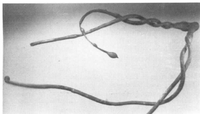
Figure 14-6.2(b) Copper conductors, fire-heated, showing beads, necking, and a pointed end.
