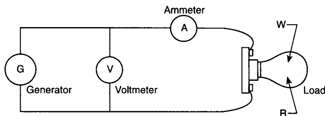
Figure 14-2.14 The power, in watts (P), consumed by a light bulb is a product of the current (I) squared and the resistance (R) of the light bulb.
