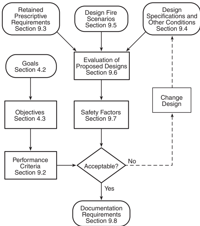
Δ FIGURE G.1 Performance-Based Fire Safety Code Compliance Process. [101:A.5.1.1]
