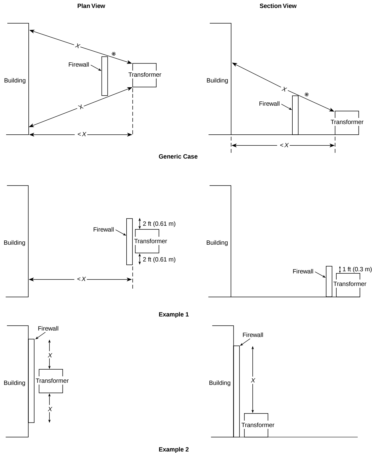
FIGURE 3-2.2.3 Illustration of oil-insulated transformer separation recommendations.
