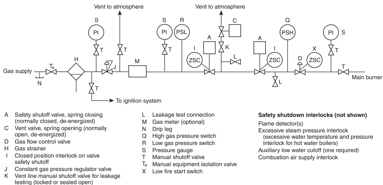
FIGURE A.5.4.2.3 Typical Fuel Supply Systems and Safety Controls for Gas Burner.
