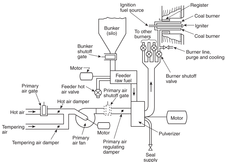
FIGURE A.6.8.5.1.5.4(b) Typical Direct-Fired Pulverizing Subsystem, Individual External Transport Type.
