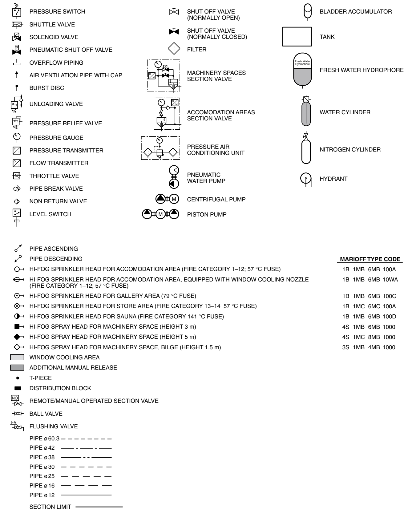
FIGURE 8-1.3(e) Legend for typical water mist plans. (Courtesy of Marioff.)
