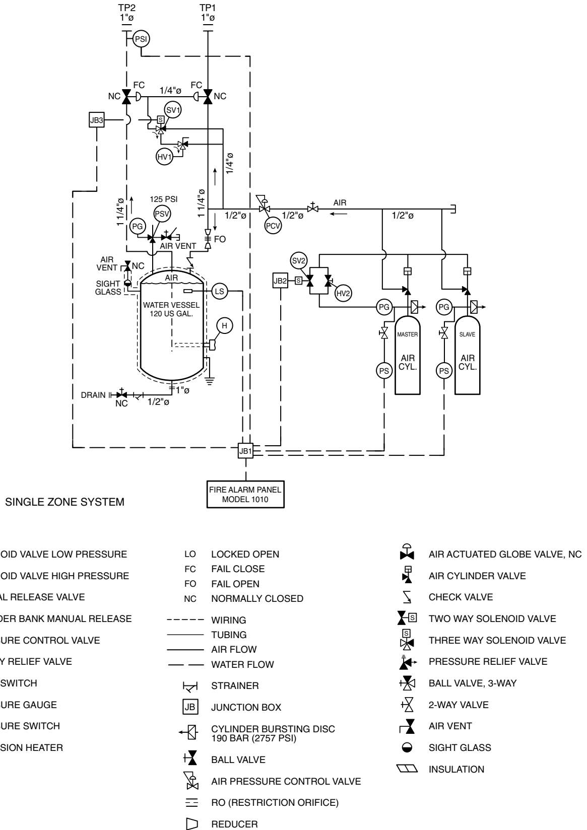
FIGURE 8-1.3(a) Typical water mist plans. (Courtesy of Securiplex.)
