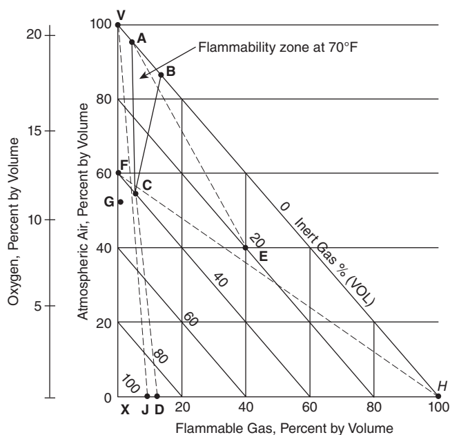
Figure 2-2 Flammability End-point Diagram Air – Flammable Gas (Methane) – Inert Gas (Nitrogen)
