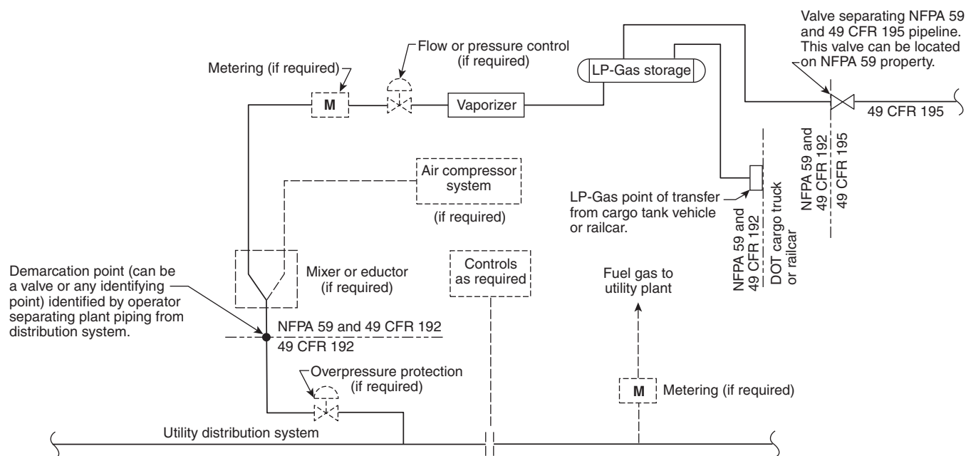
▲ FIGURE A.1.1.2(6) Typical Installation of an LP-Gas or an LP-Gas Air Facility. [59:Figure A.1.1.1]
