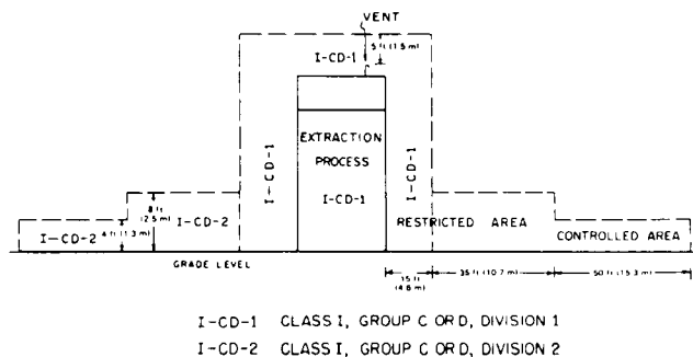
Figure 2 Type and Extent of Hazardous Areas.
