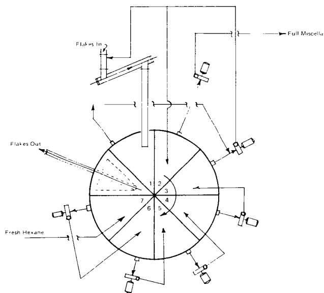
Figure A-5 Rotary Extractor.
