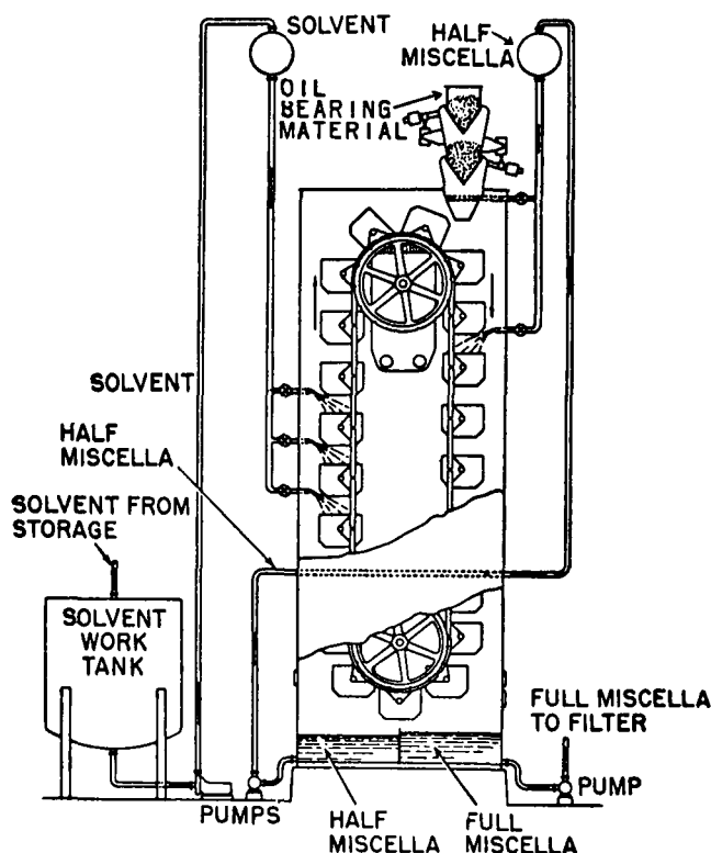
Figure A-2 Vertical Basket Extractor.
