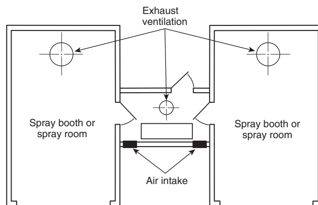
FIGURE 8.3.5(a) Mixing Room Within 1830 mm (6 ft) of Spray Area, Including Maximum Volume of Liquid Allowed.
