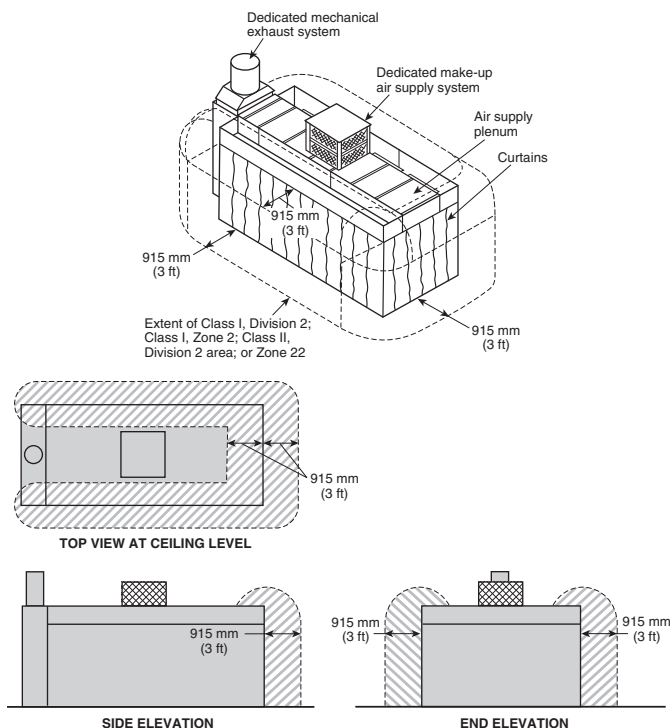
FIGURE 14.3.5.1 Class I, Division 2; Class I, Zone 2; Class II, Division 2; or Zone 22 Locations Adjacent to a Limited Finishing Workstation.
