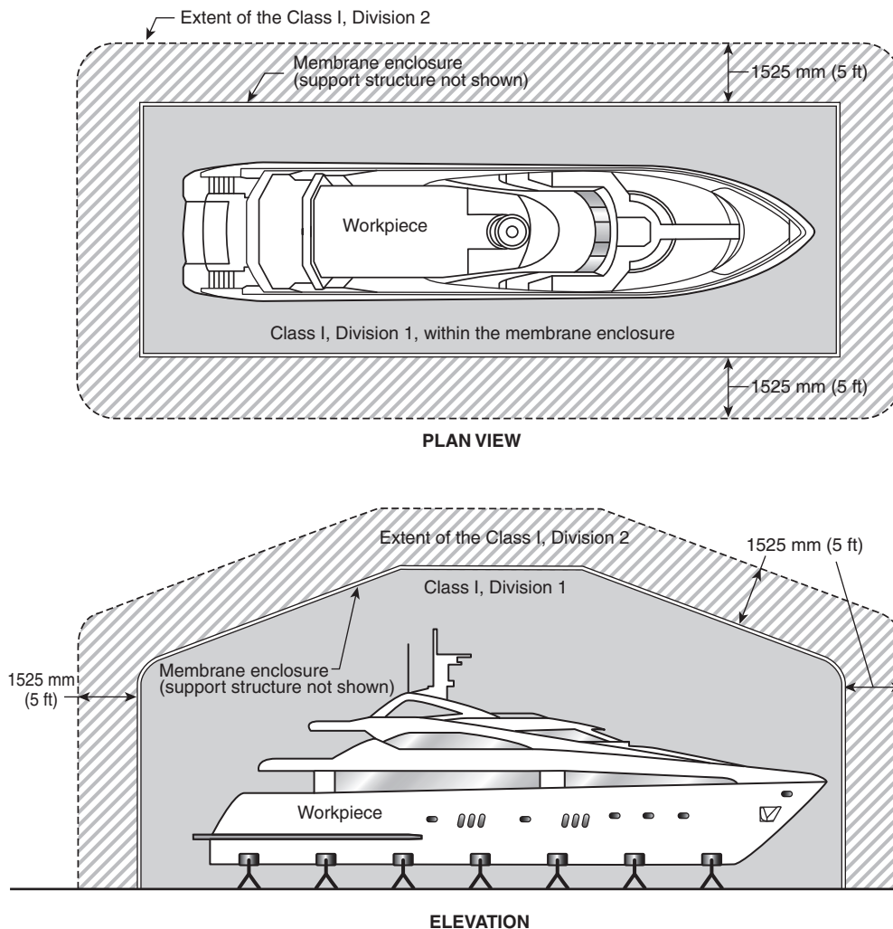
FIGURE 18.7.1.1 Electrical Classifications for Outdoor Membrane Enclosures.
