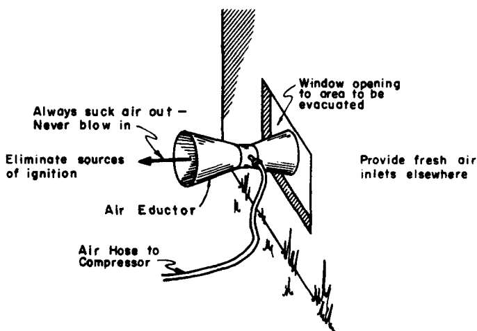
Figure 1 Exhaust Venting
