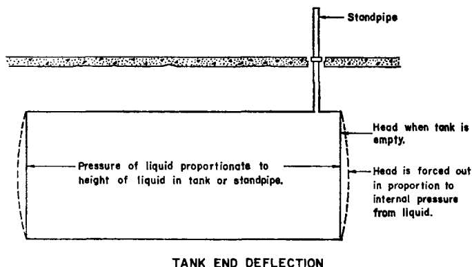
Figure 5 Tank End Deflection
