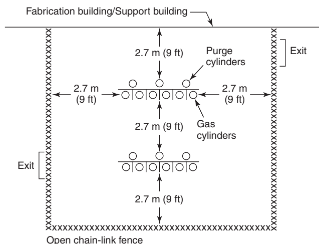
FIGURE 8.4.3 Silane Dispensing Area.
