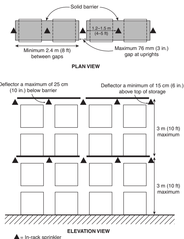
FIGURE 6.6.1.1(a) Single-Row Rack Sprinkler Layout for Design Scheme A.
