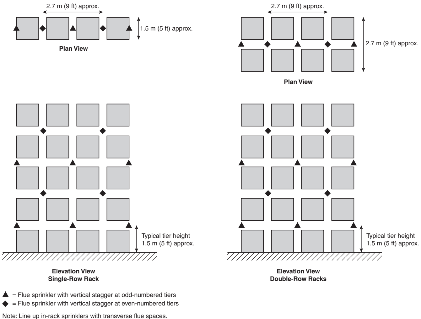
▲ FIGURE 6.4.2.7(a) In-Rack Sprinkler Layout, Cartoned Level 2 and Level 3 Aerosol Products.
