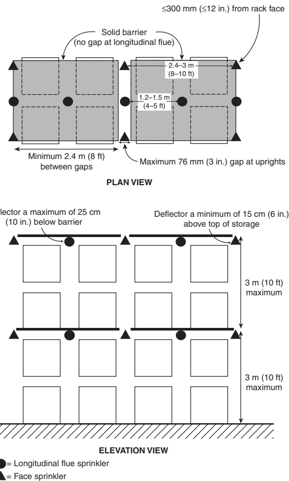
FIGURE 6.6.1.1(c) Double-Row Rack Sprinkler Layout for Design Scheme A.
