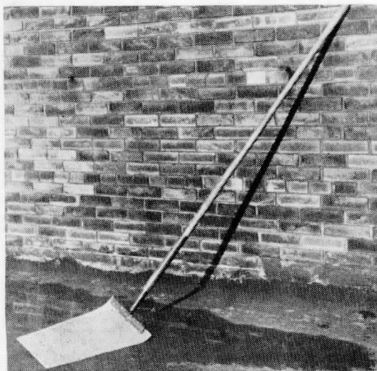
(Left) Typical swatter or flail has a wooden handle at least 60 inches long and weighs between 5 and 7 pounds.
