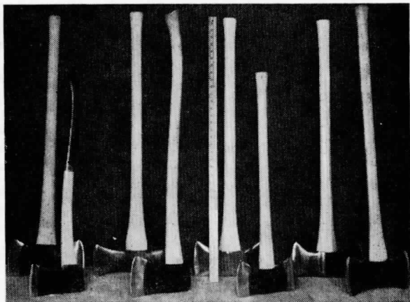
(Right) Axes: single and double bit.
