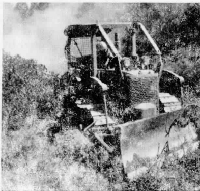
Tractor, angle dozer equipped and cable operated. Angle dozers may be positioned to operate as straight dozers. Brush guards are recommended for tractors which are to be used in the woods. All tractors should be equipped with an effective spark arrestor.
