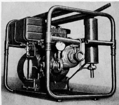
Single stage centrifugal pump in the 175-pound class. The pump is rated at 15 U.S. (12.5 Imp.) gpm at 200 psi.
