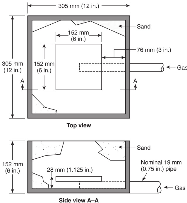
FIGURE 5.2.1 Gas Burner.
