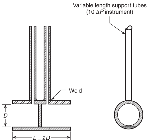
▲ FIGURE 5.4.3 Bidirectional Probe.
